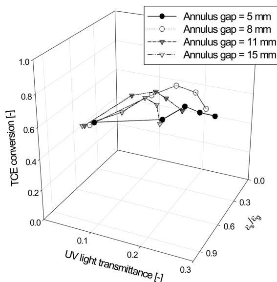
Fig. 7. Three-dimensional diagram for TCE reduction efficiency as a function of \epsilon_s/\epsilon_g and UV light transmittance with a variation of annulus gap.
